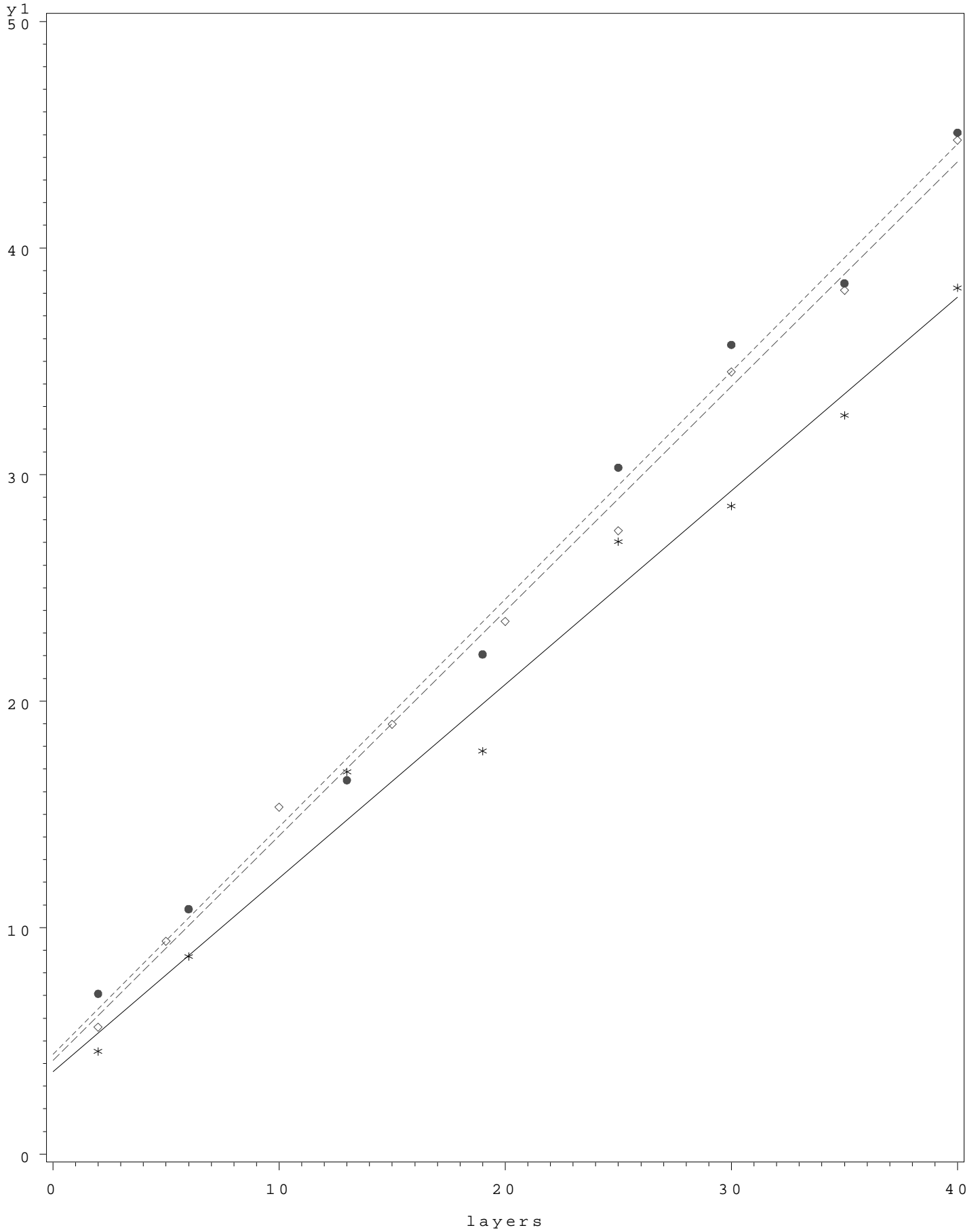
V50 2 versus Layers by Bullet Type
