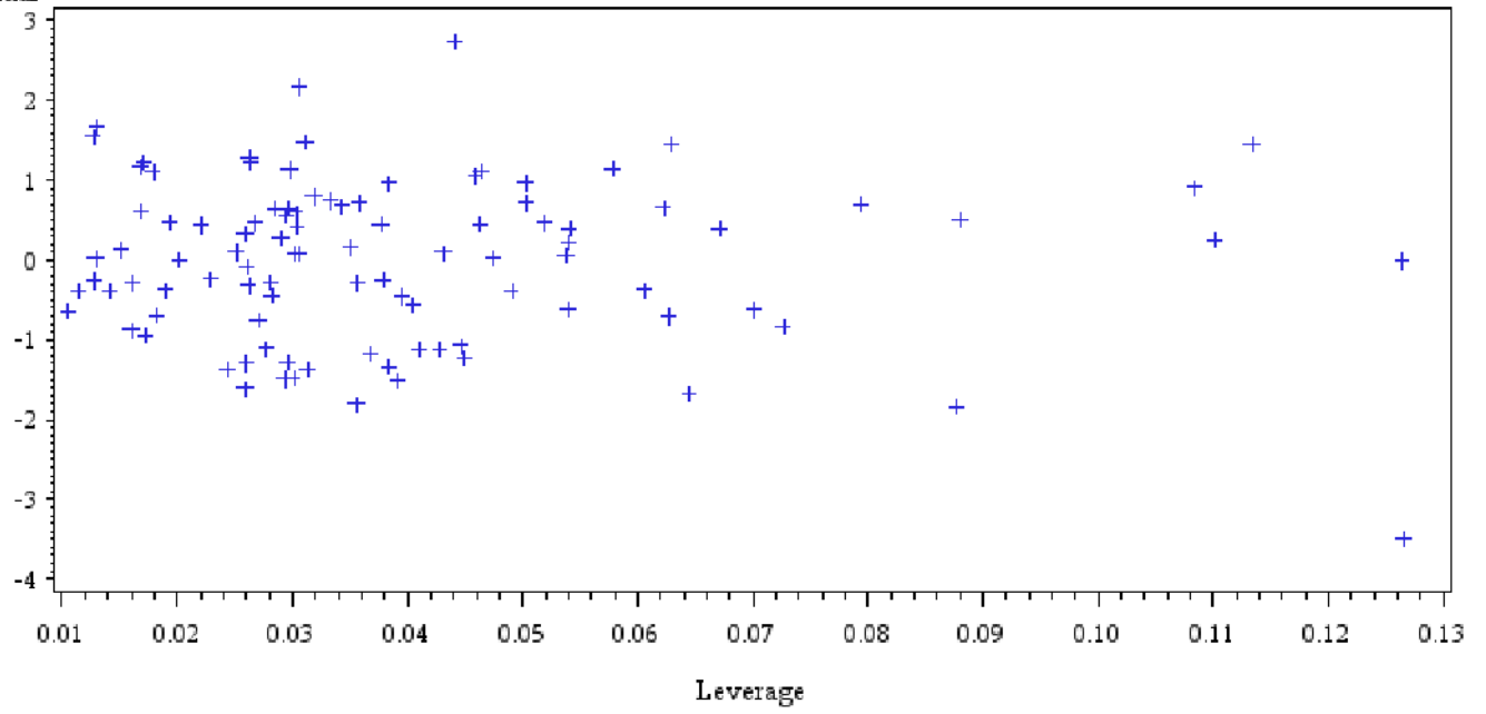
Studentized Residual
