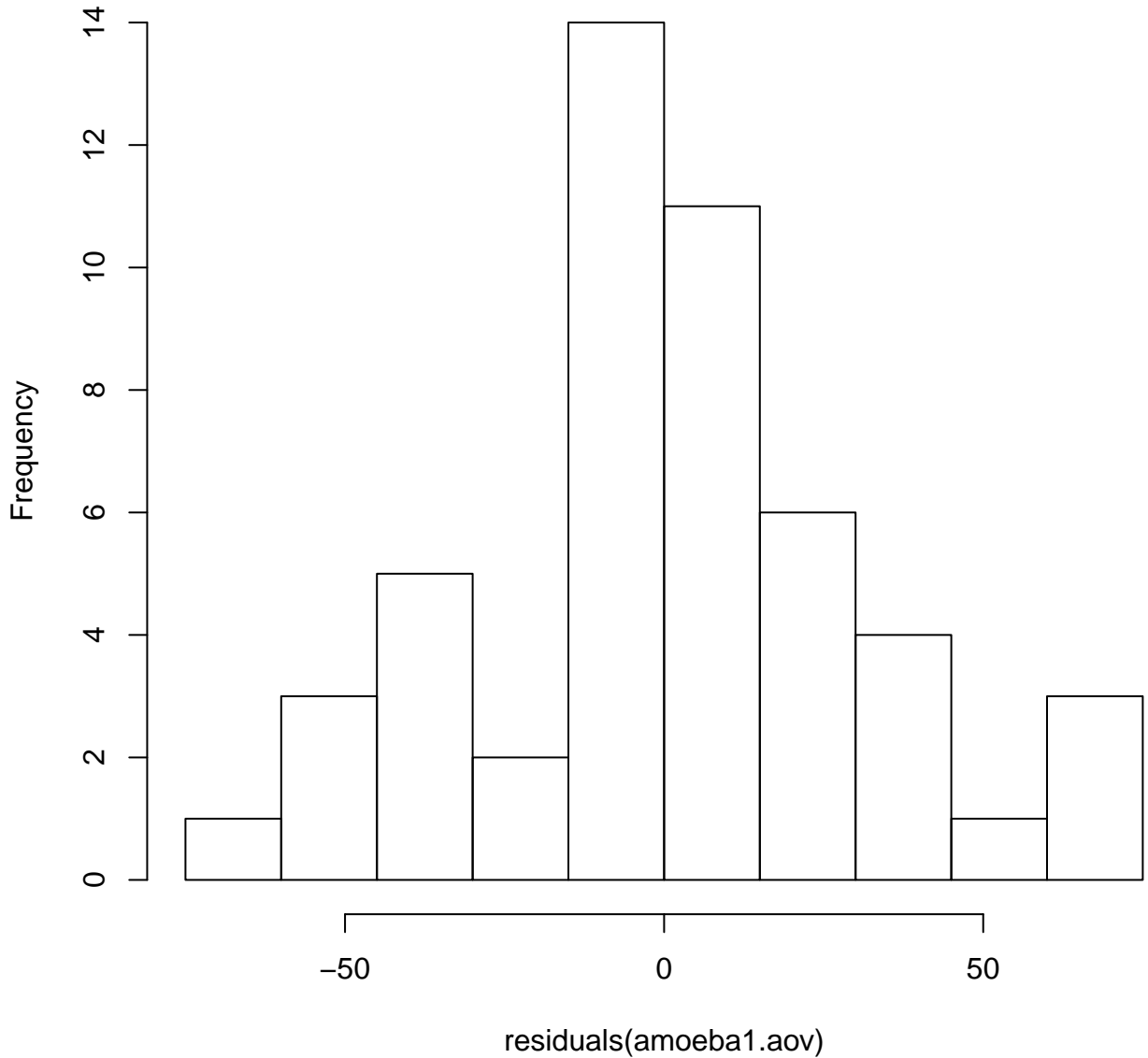
Histogram of residuals(amoeba1.aov)
