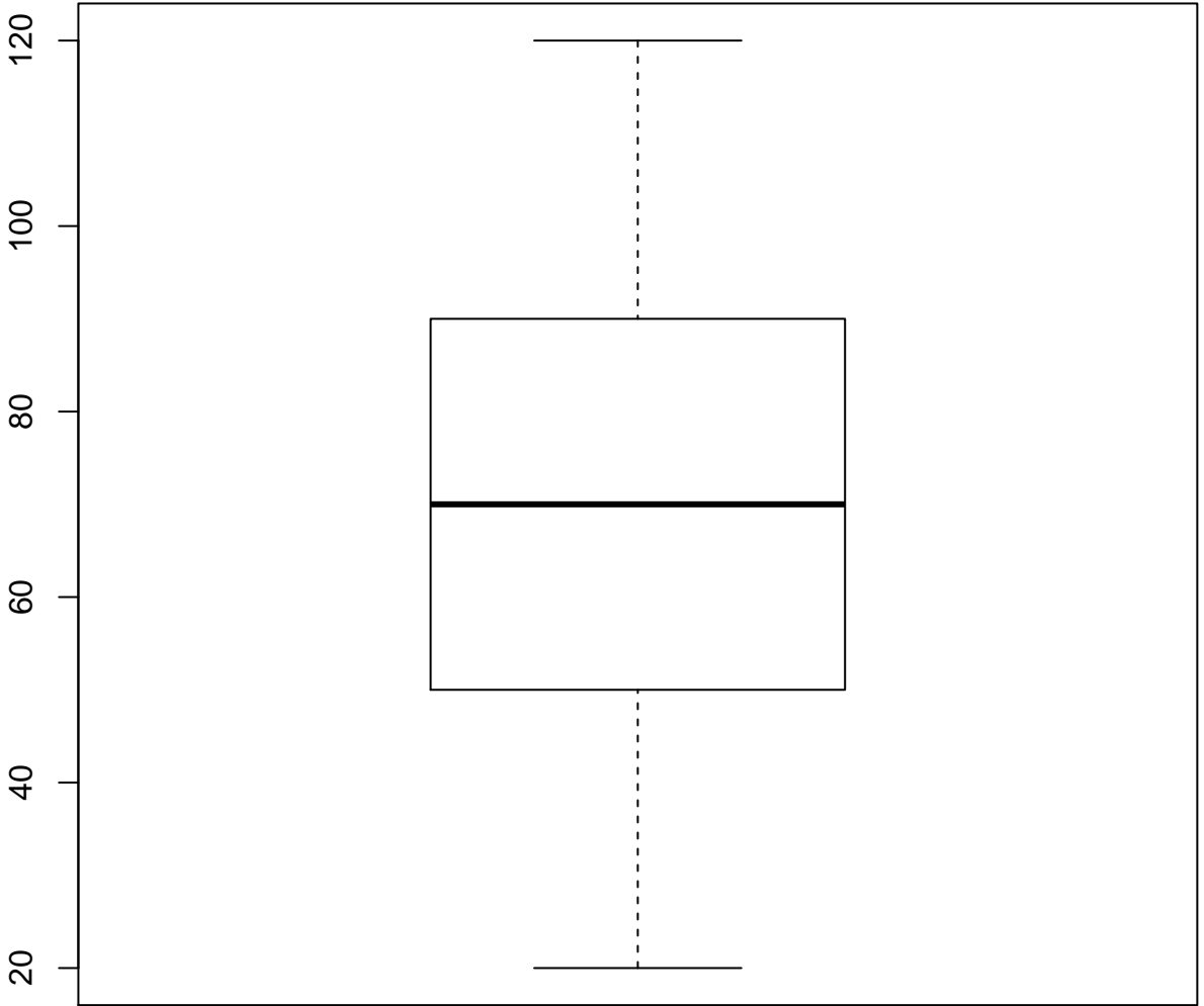
Boxplot of X
