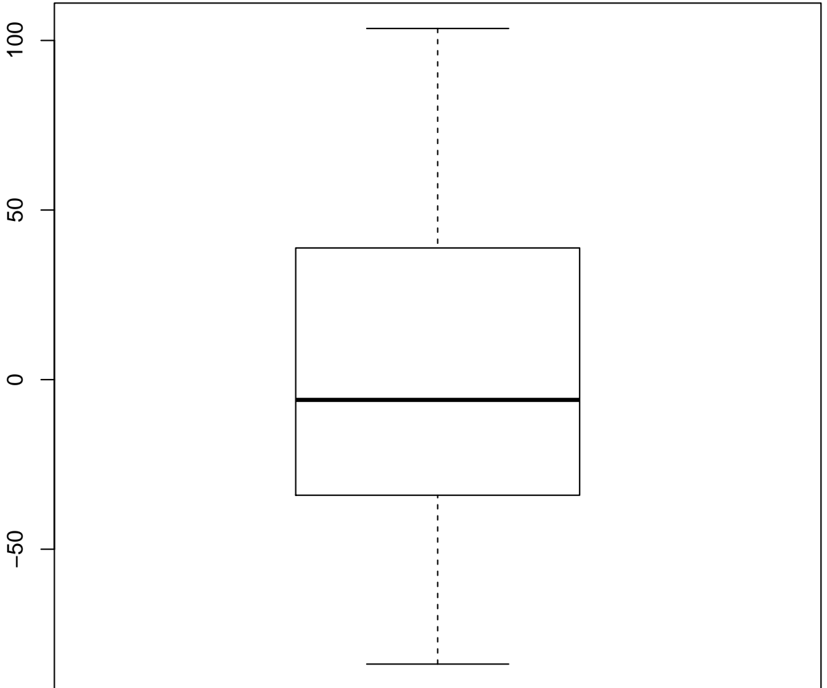
Residual boxplot
