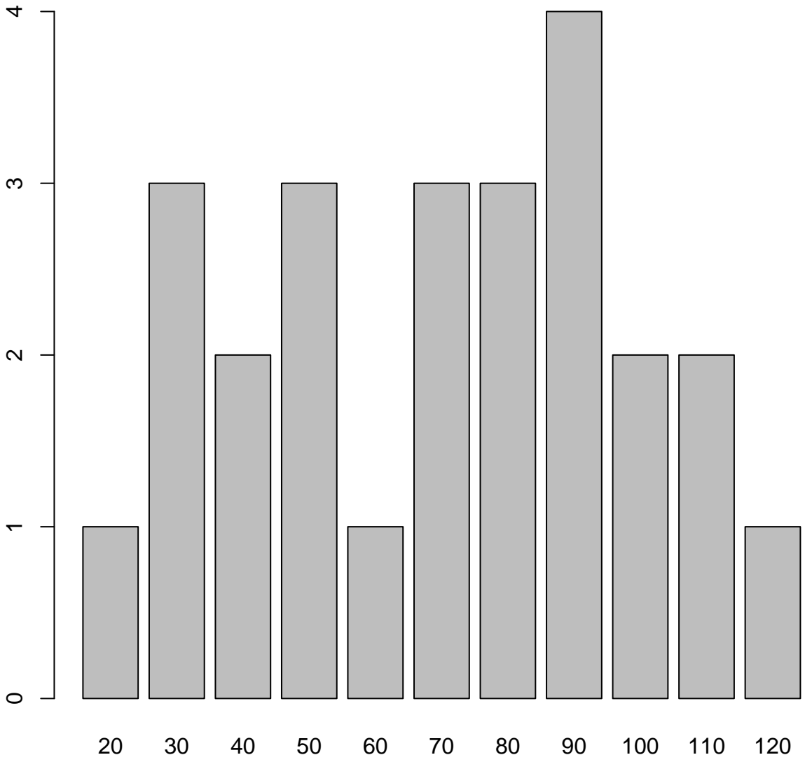
Barplot of X Levels
