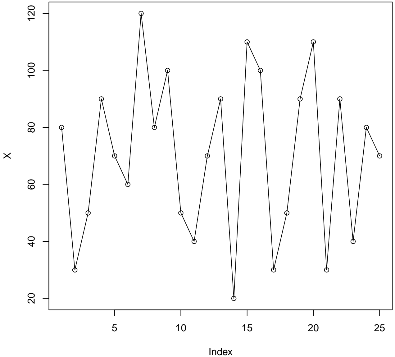
X vs Run Number
